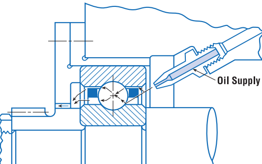
Fig. 15. Jet lubrication system.
