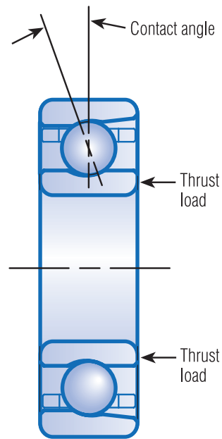
Fig. 4. Contact angle refers to the nominal angle between the ball-to-race contact line and a plane through the ball centers, perpendicular to the bearing axis.
