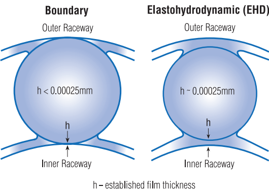
Fig. 13. Lubrication Regimes.
