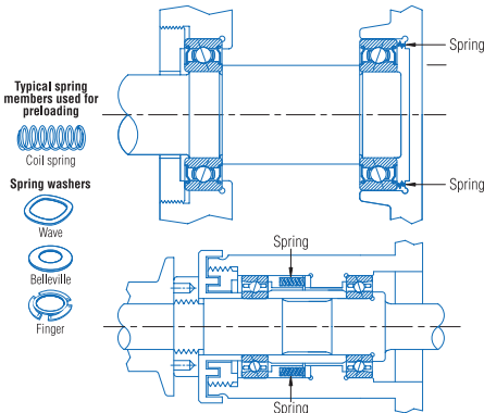
Fig. 6. Different types of spring preloading.
