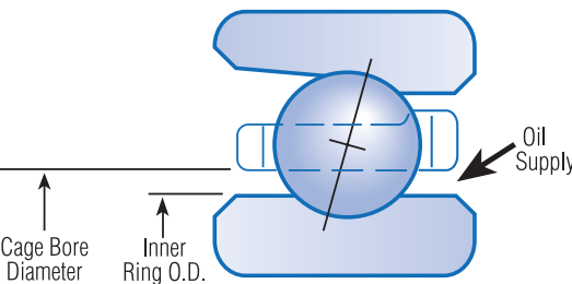
Fig. 16. Lubrication window for H-type bearing.
