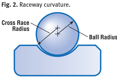
Fig. 2. Raceway curvature.
