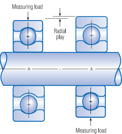
Fig. 3. Radial play is a measure of internal clearance and is influenced by measuring load and installation practices. A high radial play value is not an indication of lower quality or less precision.
