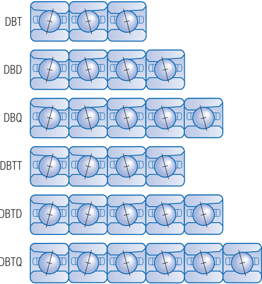
Fig. 12. Increased stiffness can be achieved by mounting bearings in sets.
