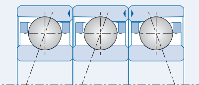
TBT arrangement <<>
