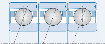
TDT arrangement <<<
