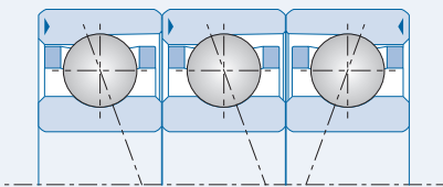
TFT arrangement >><
